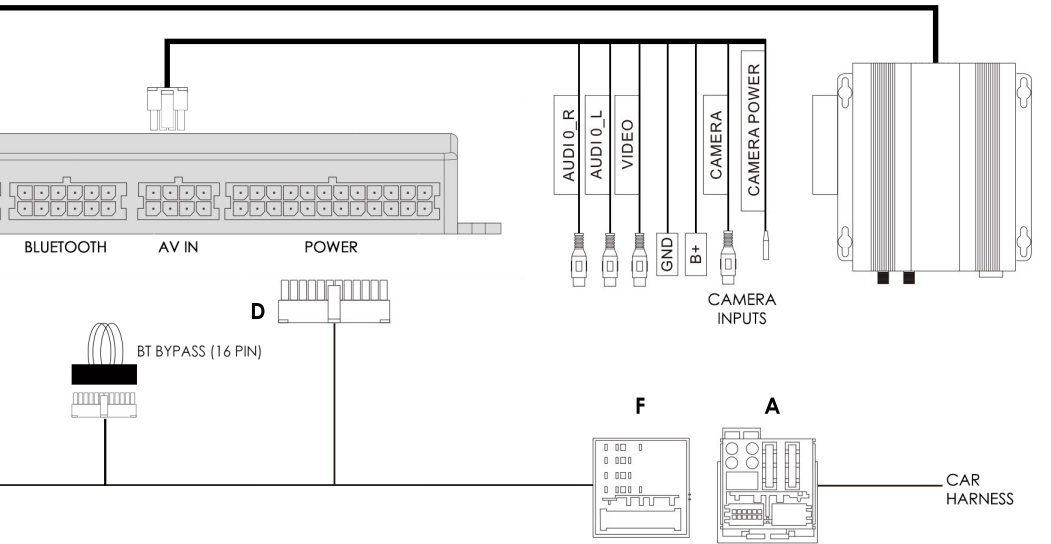
DVBT INTERFACE (NOT INCLUDED) PART NUMBER: ADV-DVBT
